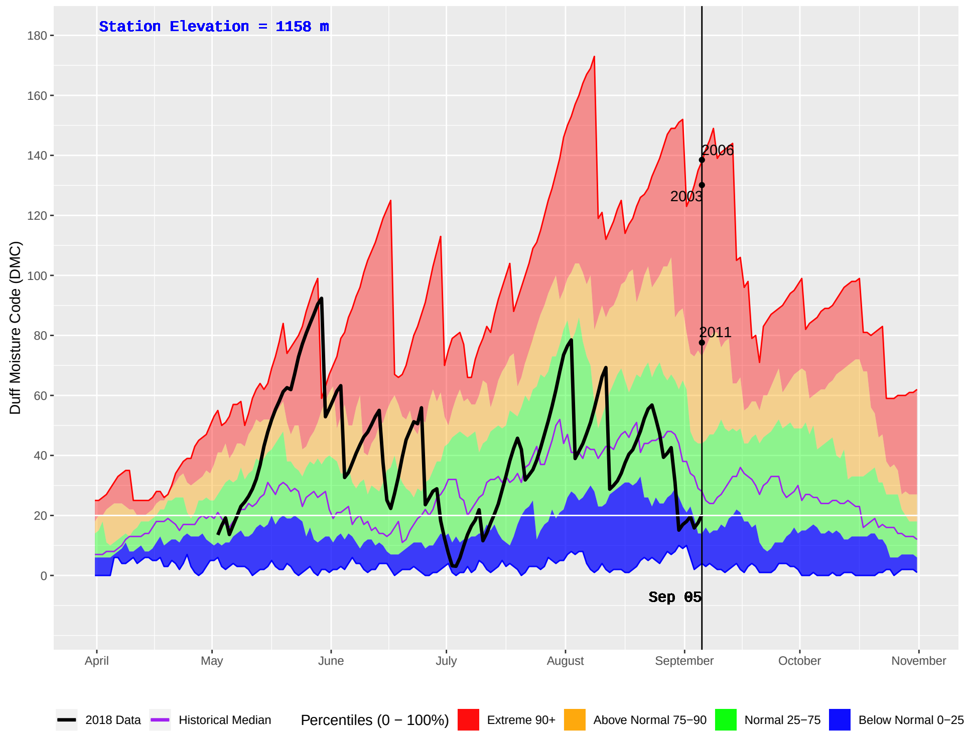
LONE BUTTE (218) : Historical (1987–2016) and Current (2018) Daily Duff Moisture Code (DMC)
