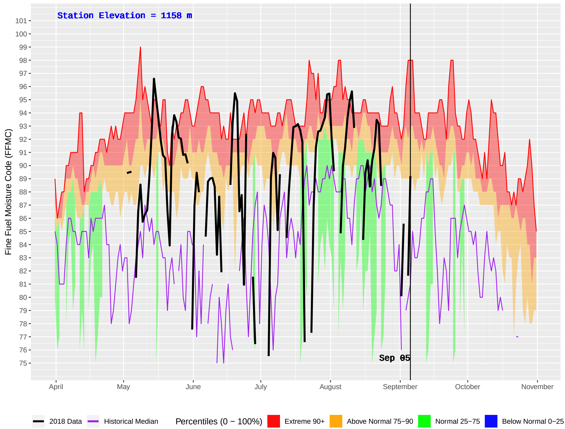
LONE BUTTE (218) : Historical (1987–2016) and Current (2018) Daily Fine Fuel Moisture Code (FFMC)
