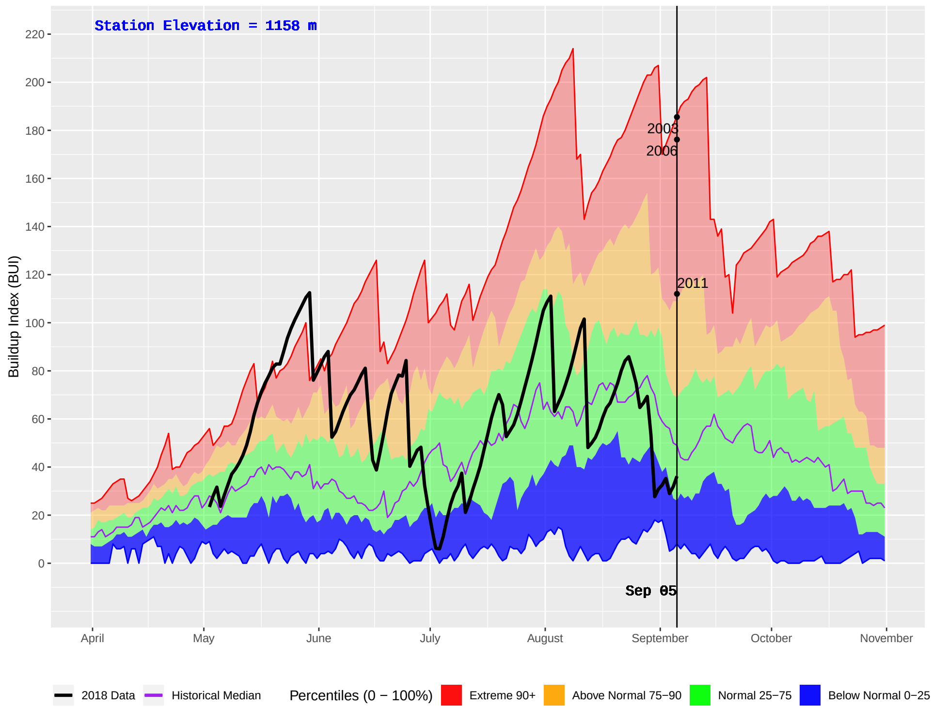
LONE BUTTE (218) : Historical (1987–2016) and Current (2018) Daily Buildup Index (BUI)
