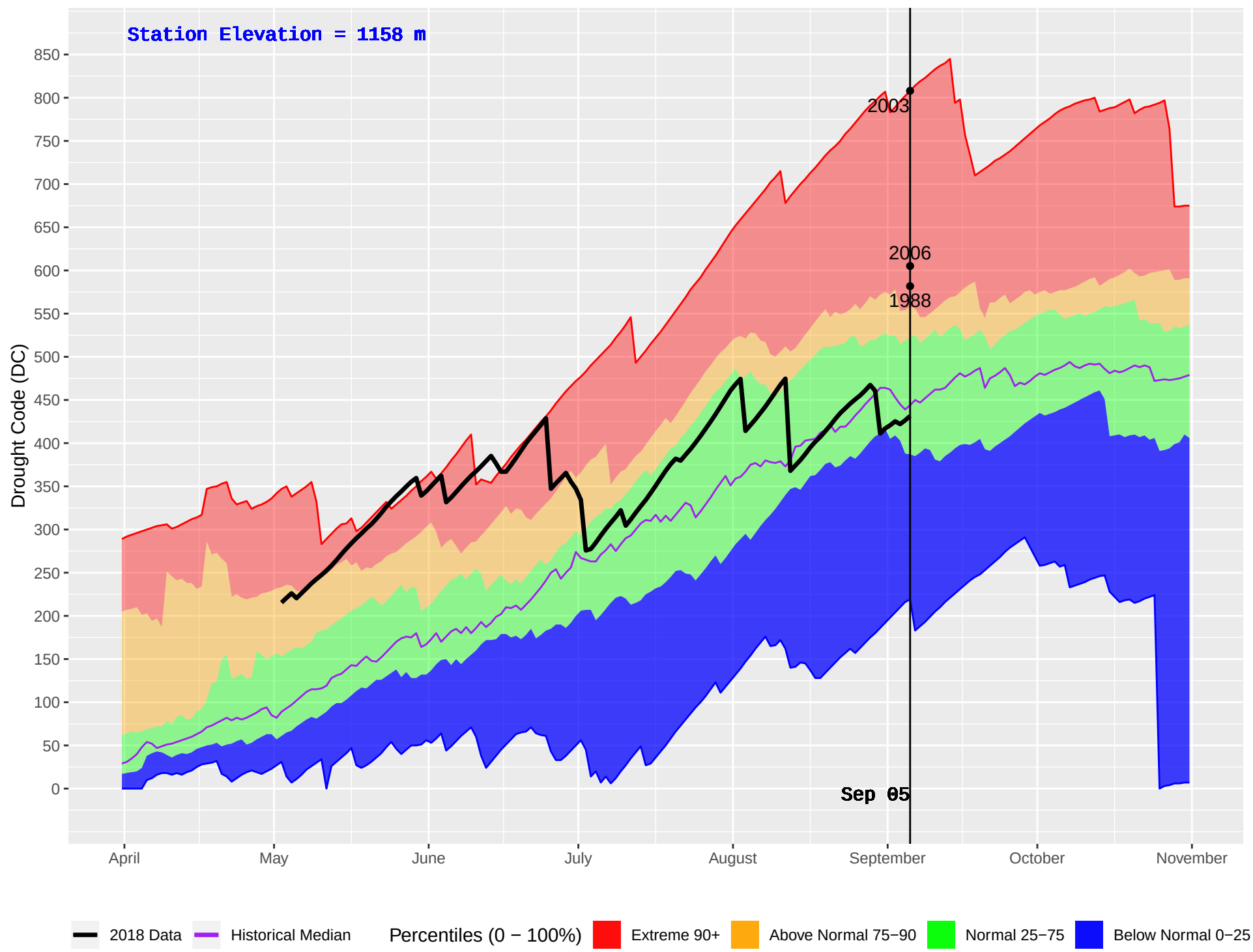
LONE BUTTE (218) : Historical (1987–2016) and Current (2018) Daily Drought Code (DC)
