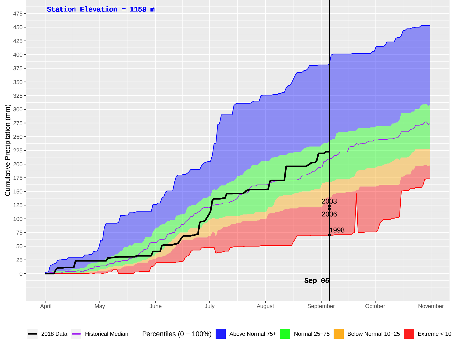
LONE BUTTE (218) : Historical (1987–2016) and Current (2018) Daily Cumulative Precipitation
