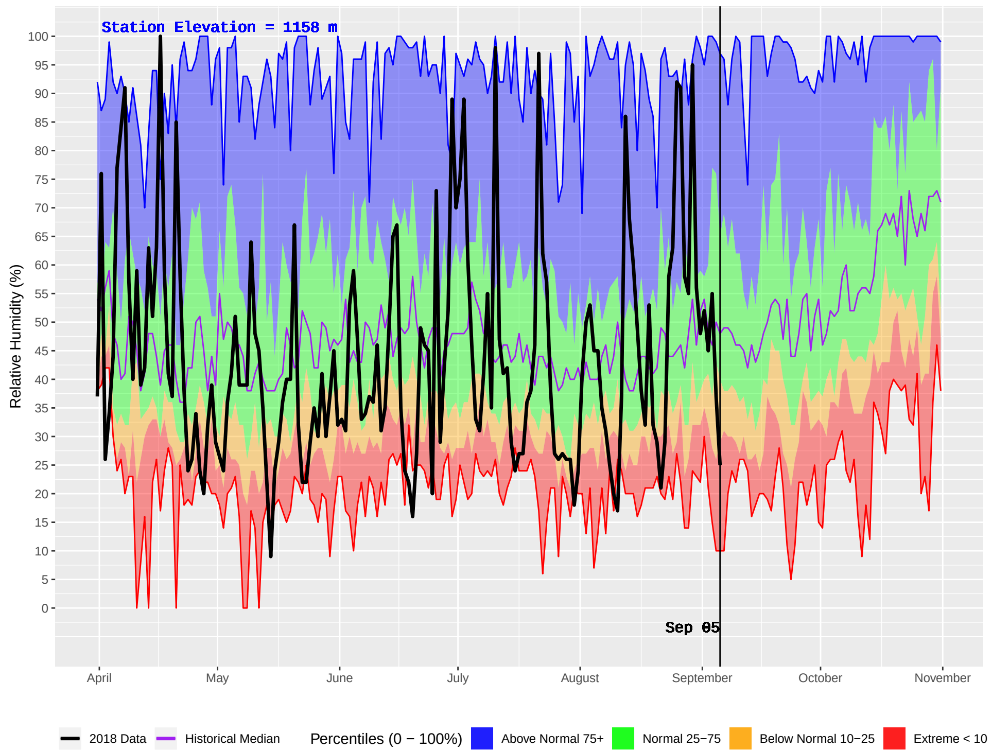
LONE BUTTE (218) : Historical (1987–2016) and Current (2018) Daily Relative Humidity
